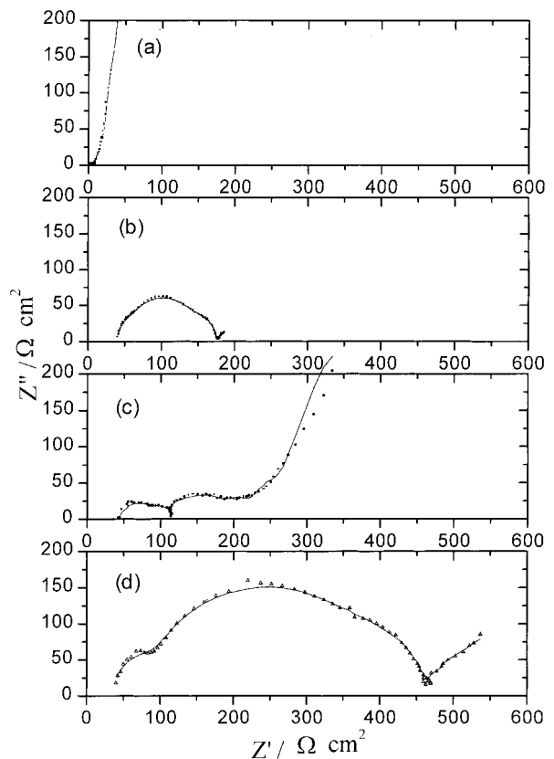
Fig. 4. Nyquist plot measured at OCV: (a) 3.1, (b) 0.54, (c) 0.24 and (d) 0.05 V vs Li/Li + in DMC/1 M LiPF 6 electrolyte.
