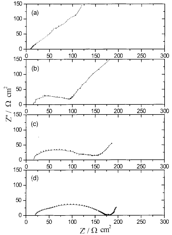
Fig. 6. Nyquist plot measured at OCV: (a) 3.1, (b) 0.61, (c) 0.25 and (d) 0.05 V vs Li/L + in EC/DMC/1 M LiPF 6 electrolyte.
