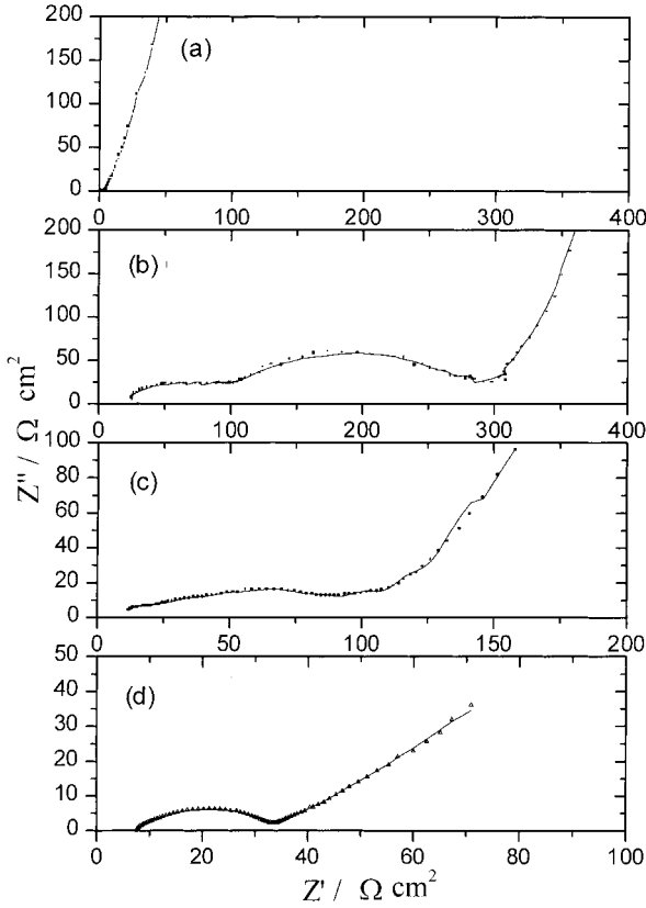
Fig. 5. Nyquist plot measured at OCV: (a) 3.1, (b) 0.65, (c) 0.23 and (d) 0.05 V vs Li/L + in EC/DEC/1 M LiPF 6 electrolyte.
